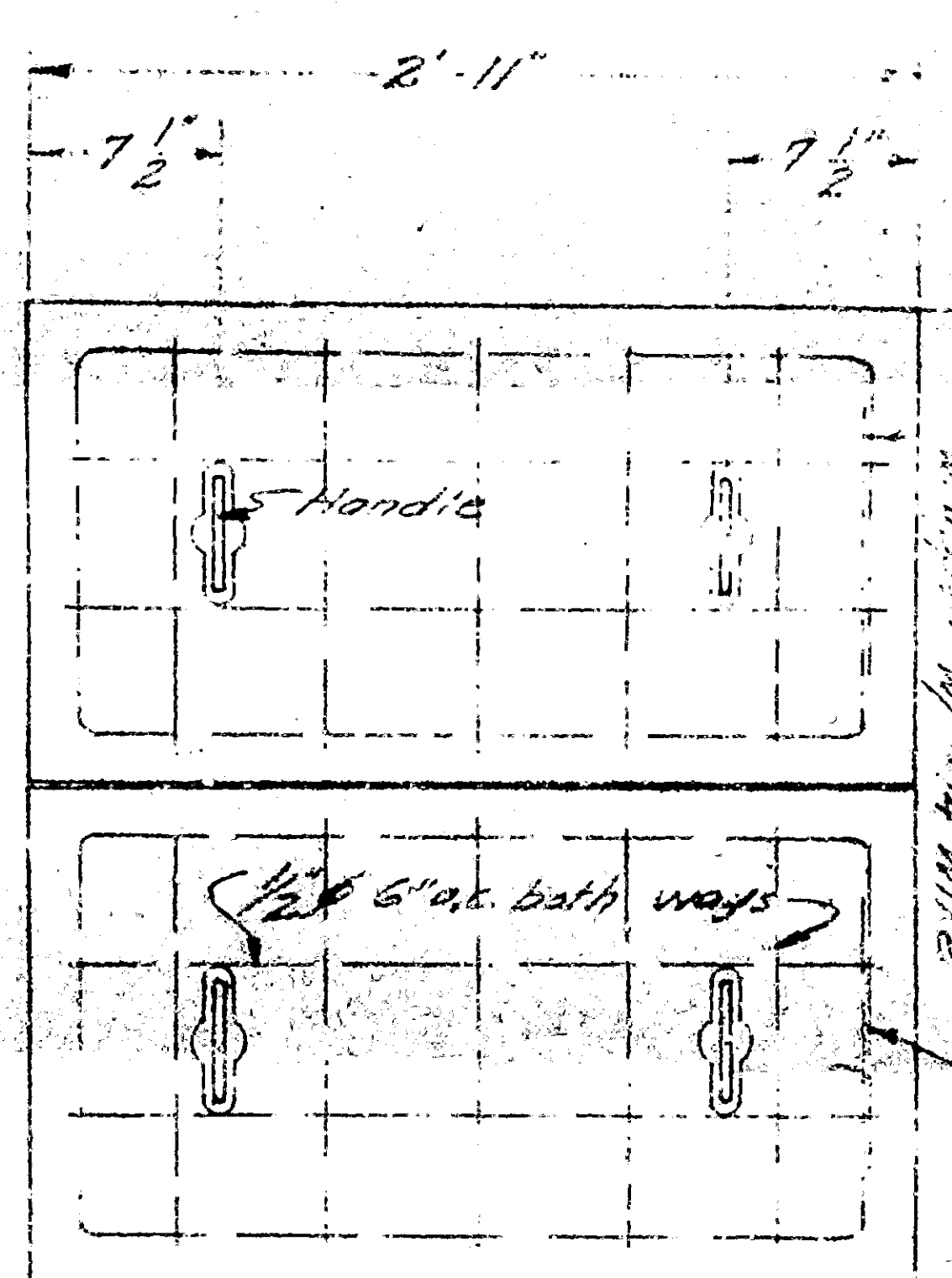
STANDARD CONCRETE COVER DETAILS SCALE 1/4"=1'-0"
